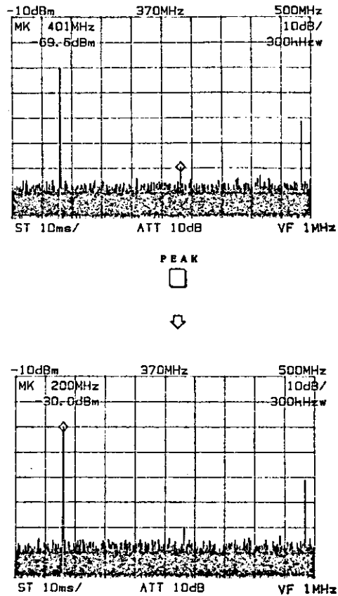
Figure 4-12 PEAK Search
