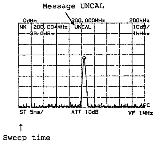
Figure 4-18 Sweep Time
