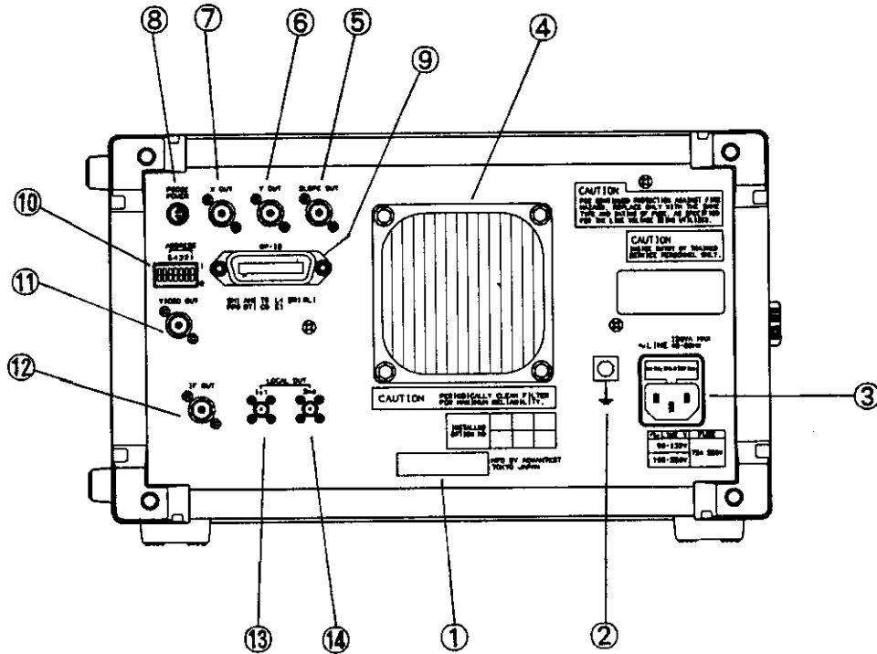
Figure 3-4 Rear Panel
