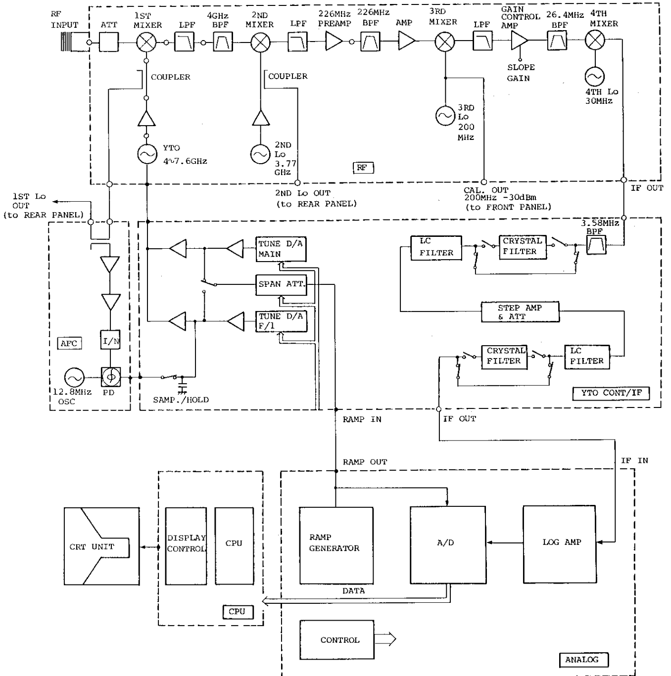
Figure 12-4 Block Diagram
