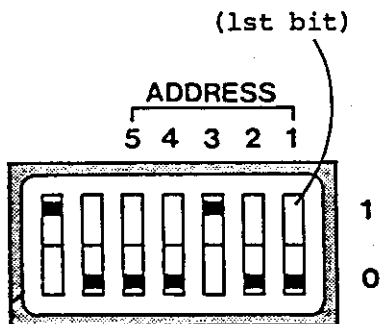
Figure 6-4 ADDRESS Switch
