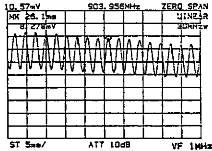
Figure 5-7 Reading the Emax
