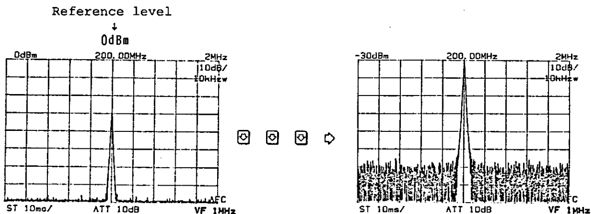
Figure 4-7 Change in Reference Level
