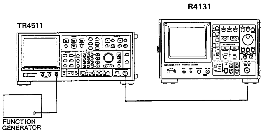
Figure 11-2 Frequency Span Test Setup
