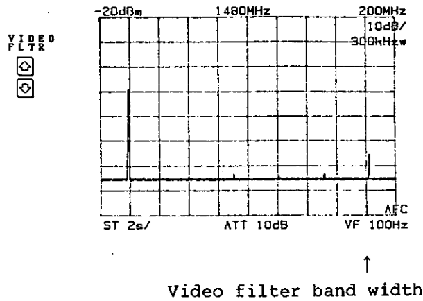
Figure 4-17 VIDEO FiLTeR
